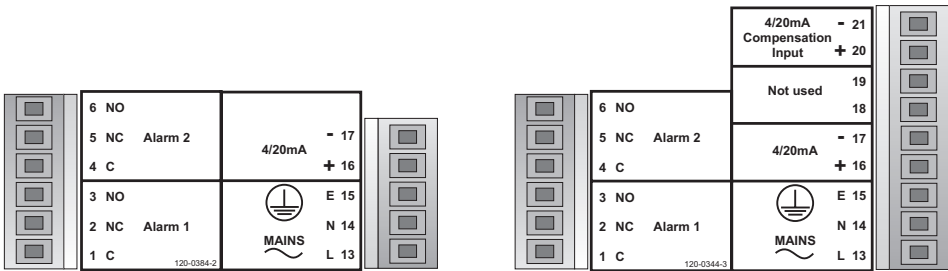
Figure 7a- Standard connections
